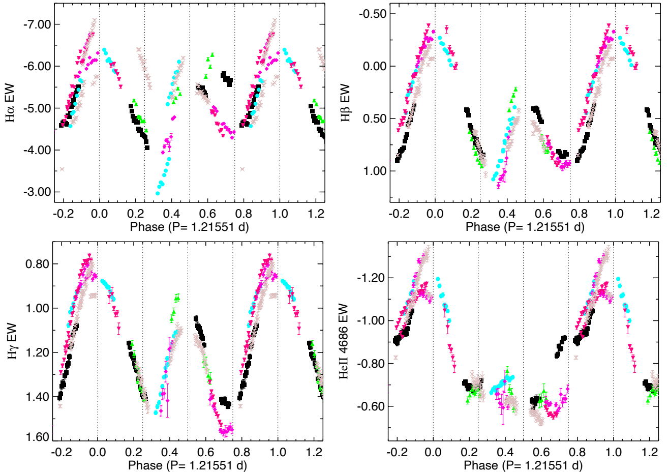
Figure 10. Phased EW measurements (in \text{\AA} ) from H \alpha , H \beta , H \gamma and He II \lambda 4686. The axis is inverted (EW increases downwards) to reflect the contribution from emission (emission increases upwards). Dotted lines are also included to indicate phases 0.0, 0.25, 0.5, 0.75, and 1.0. Different colours represent different epochs of observation.
