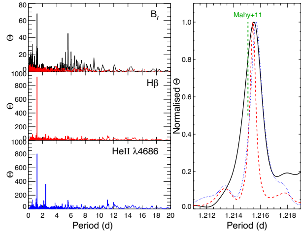
Figure 3. Periodograms obtained from the B_\ell measurements (top panel, solid black), the H\beta (middle panel, red) and the \text{He II } \lambda 4686 (bottom panel, dotted blue) EW measurements. Significant power is present in all periodograms at \sim 1.215 d. The right panel provides a narrow view of the periodograms about 1.215 d, normalised to their maximum power. The peak period identified by Mahy et al. (2011) from the CoRoT lightcurve is also indicated for comparison. Periodograms obtained from the EW measurements included contributions from the first harmonic. The panel for B_\ell (top) also presents the periodogram after prewhitening with the 1.215 d period, as discussed in the text (dashed red).
